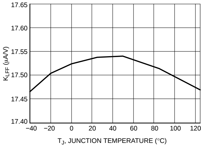
Figure 23. K LEFF vs. Junction Temperature
